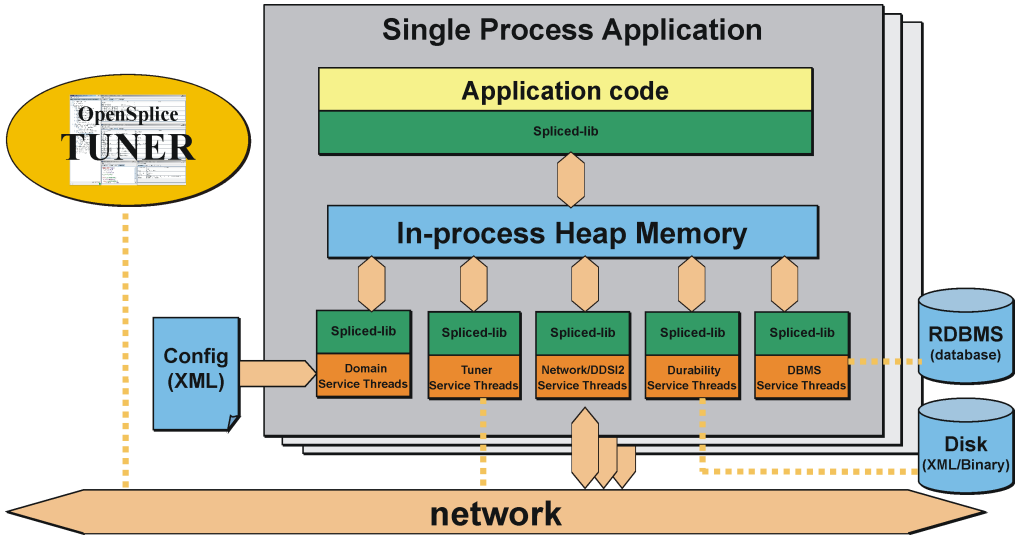
Fig. 1: The Vortex OpenSplice Single Process Architecture
