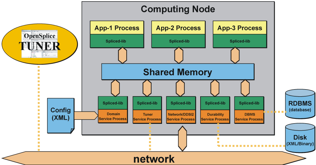
Fig. 2: The Vortex OpenSplice Shared Memory Architecture
